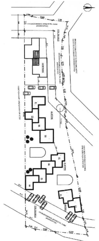
Plot Plan
