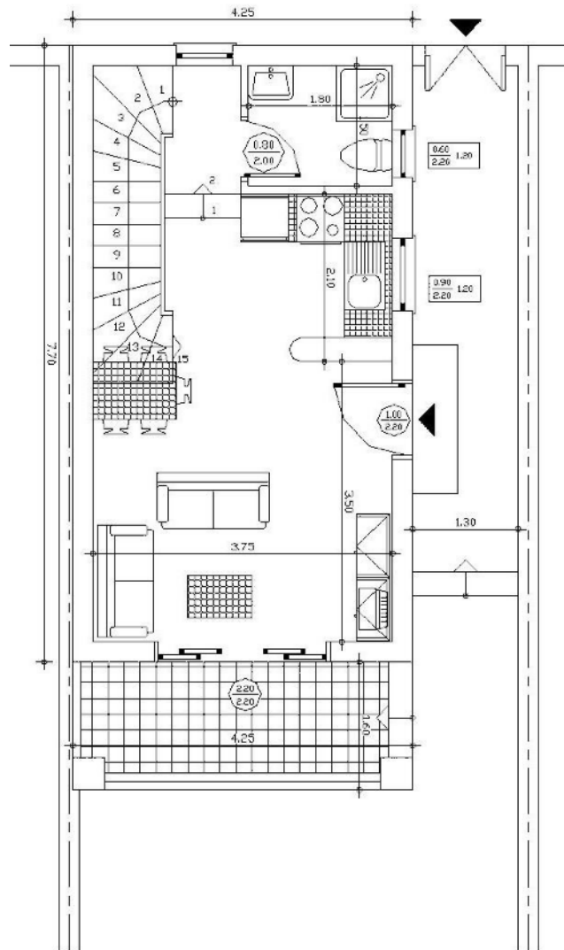
D GROUND FLOOR 32.73 m 2
